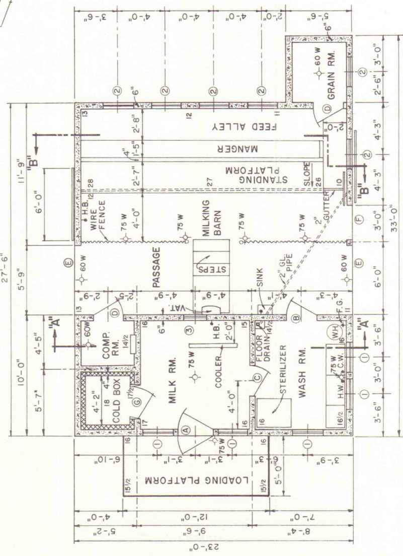
FLOOR PLAN
